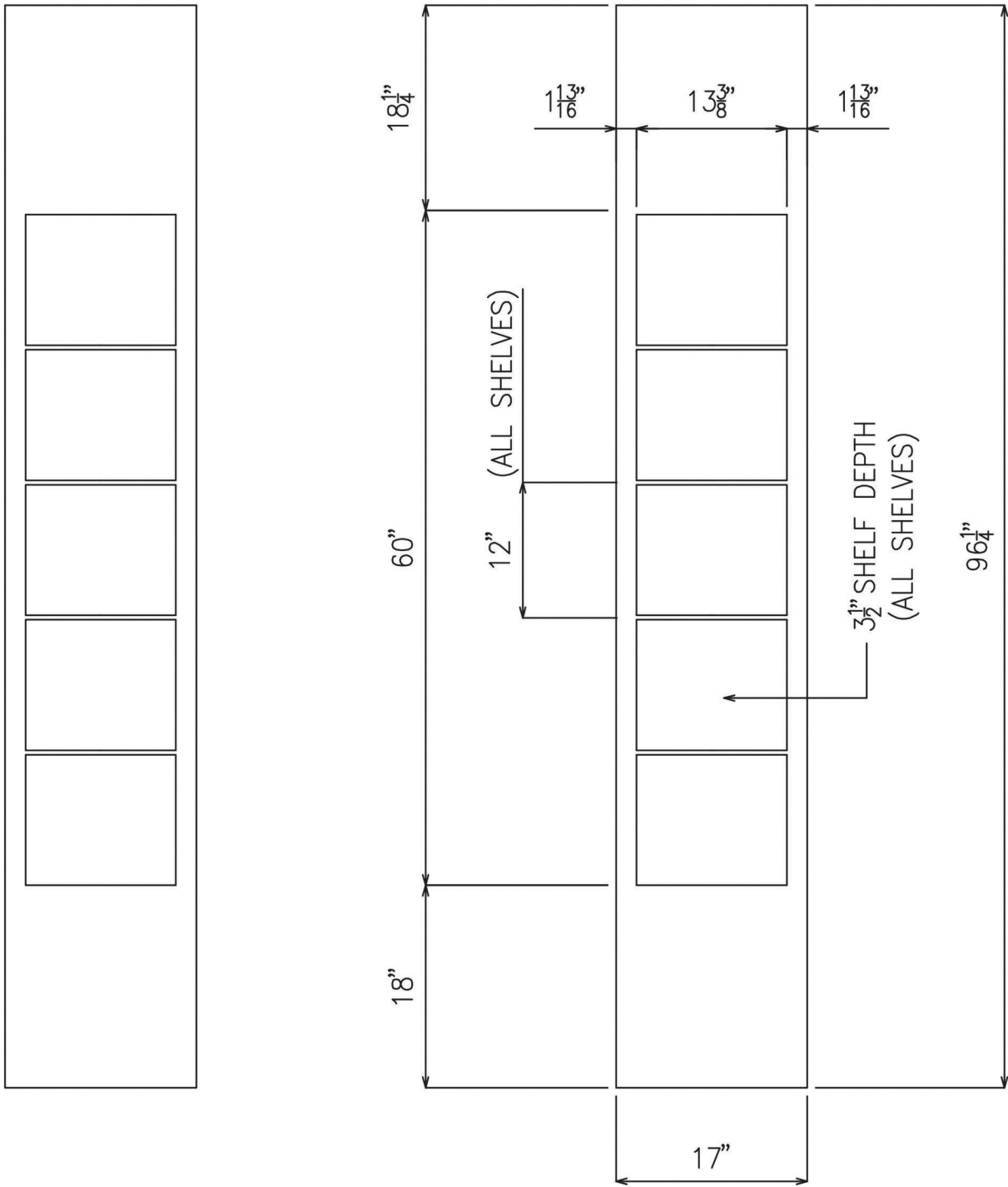
FIVE SHELF SHOWER CADDY (FRONT VIEW)
