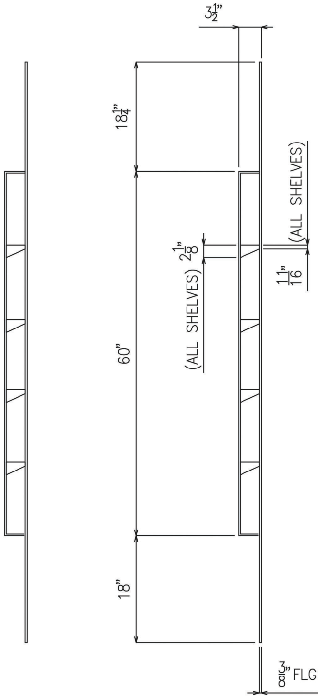
FIVE SHELF SHOWER CADDY (SIDE VIEW)
