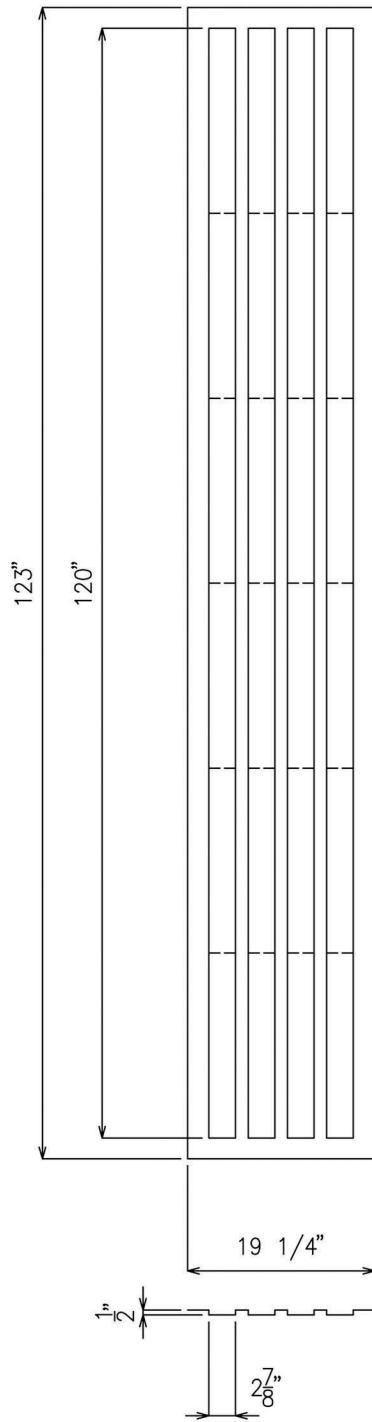
4 CAVITY PARTITIONED TRIM MOLD BM-TM03
