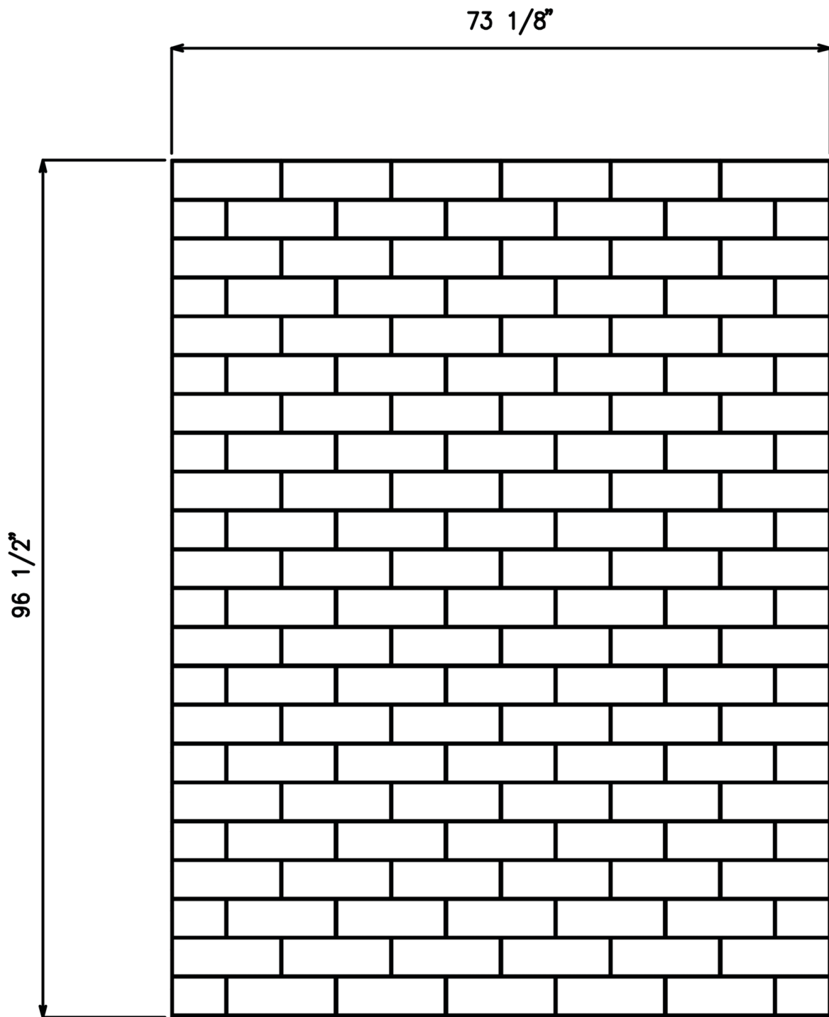
4 1/4" x 12 7/8" SUBWAY TILE MOLD BM-WP03 73 1/8" WIDE x 96 1/2" LONG
