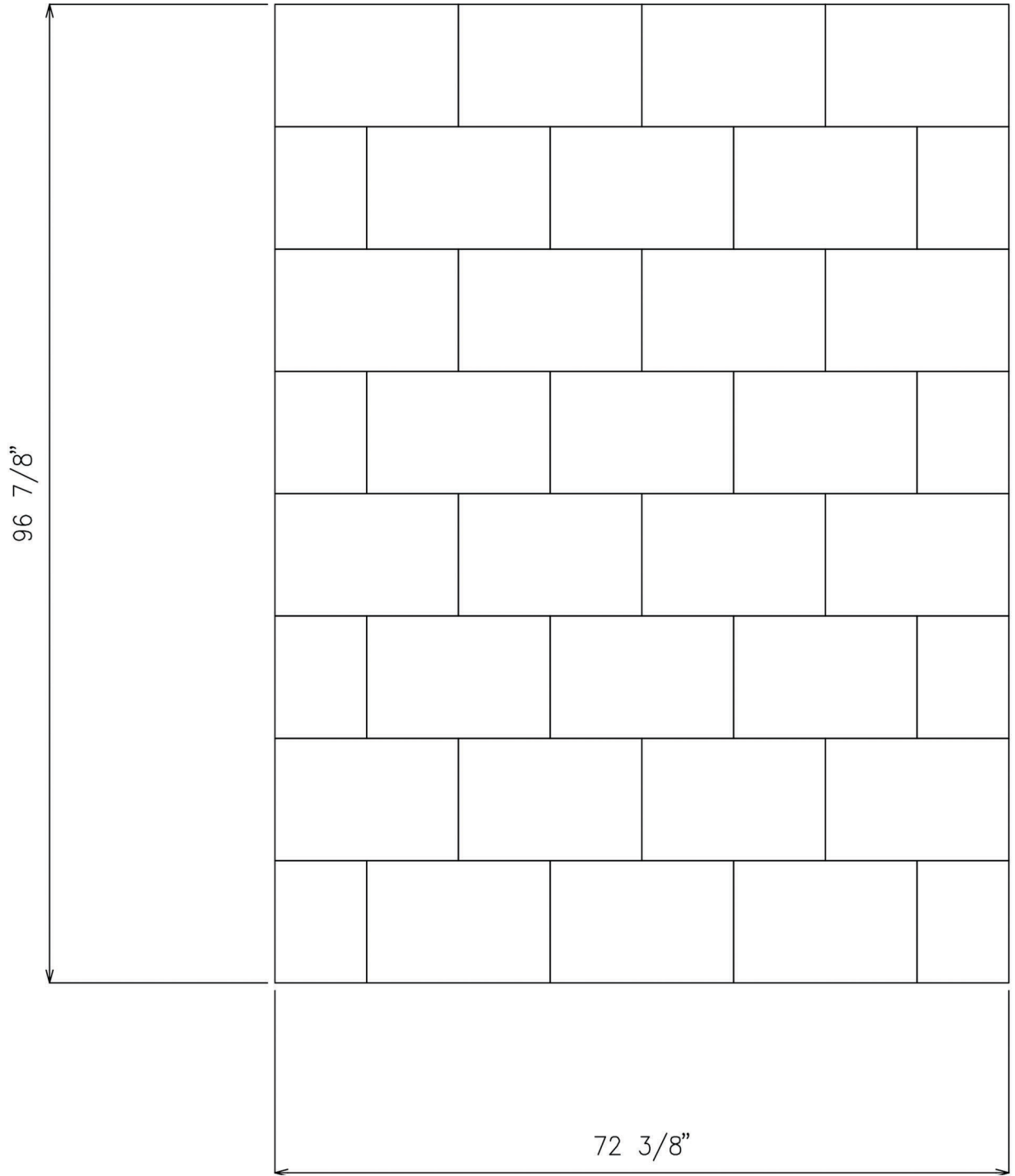
12" x 18" TILE MOLD BM-WP04 GLOSS FINISH
