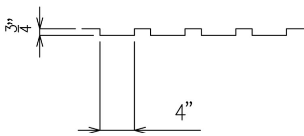
TWELVE CAVITY END SPLASH MOLD (FOR 22 1/2" TOP) ES02
